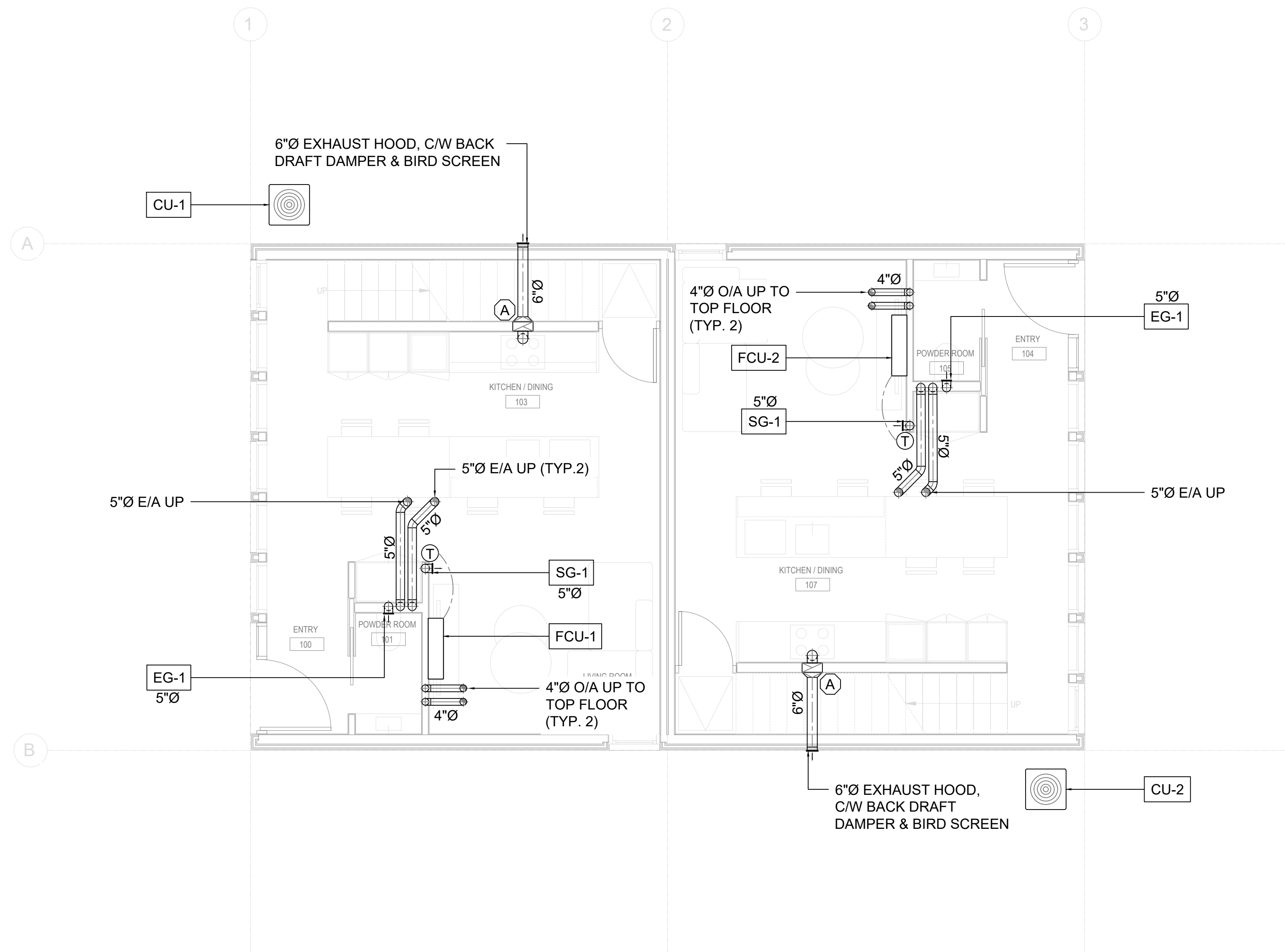
M1 LEVEL 1 FLOOR PLAN 1 1/4" : 1'
